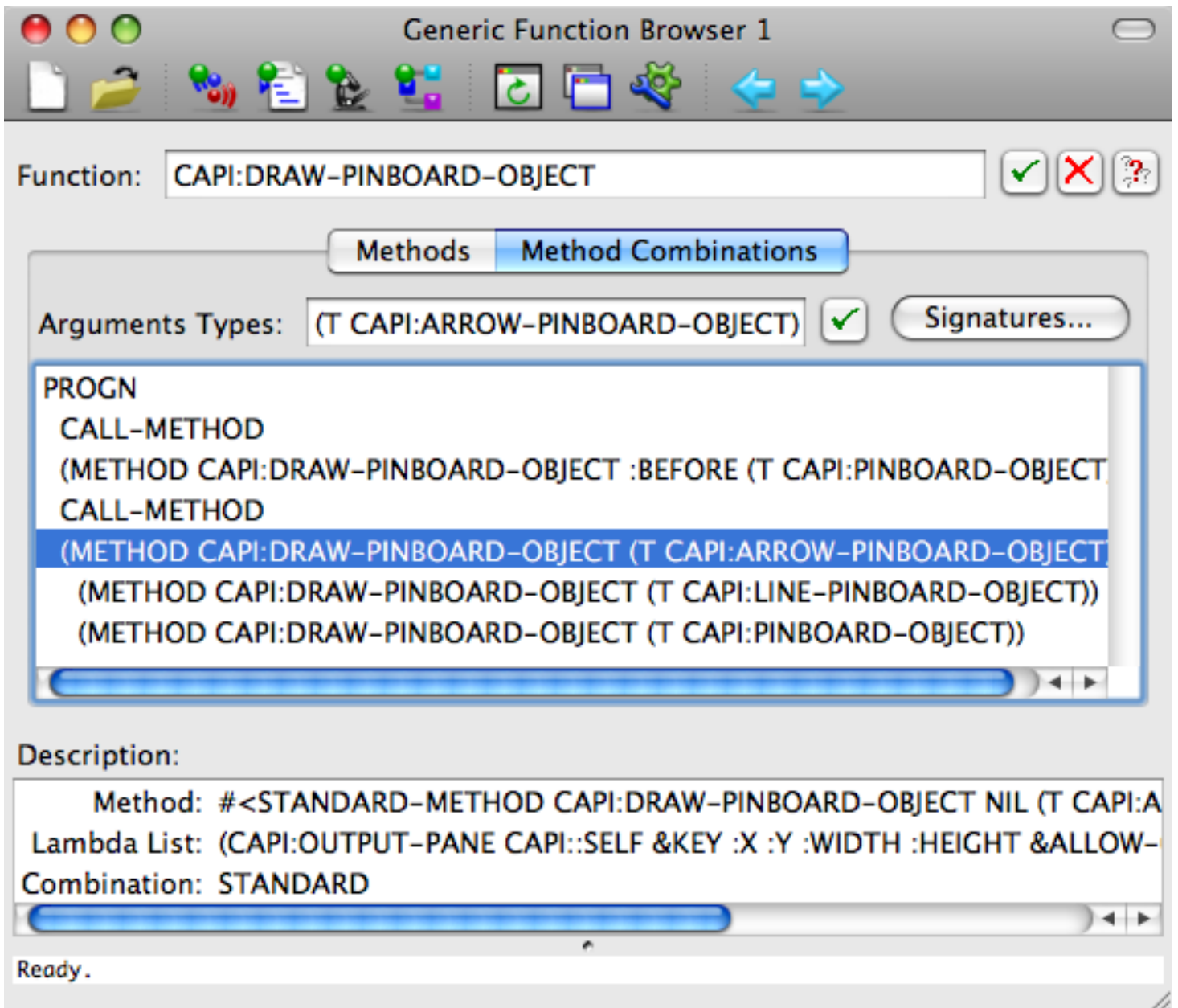
Generic function browser displaying method combinations
