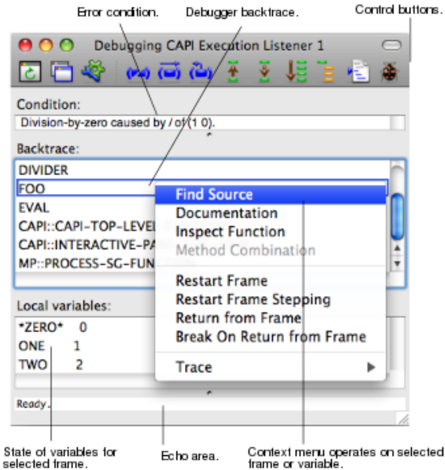
Debugger tool with two list-panels
