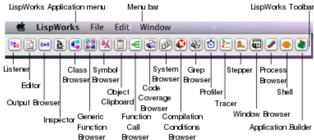
Menus and toolbar in the LispWorks IDE
