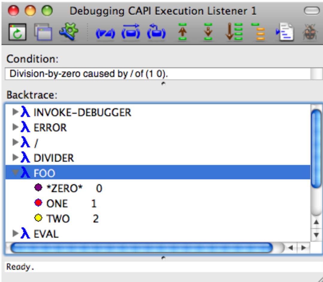
Variables in the Debugger tree view
